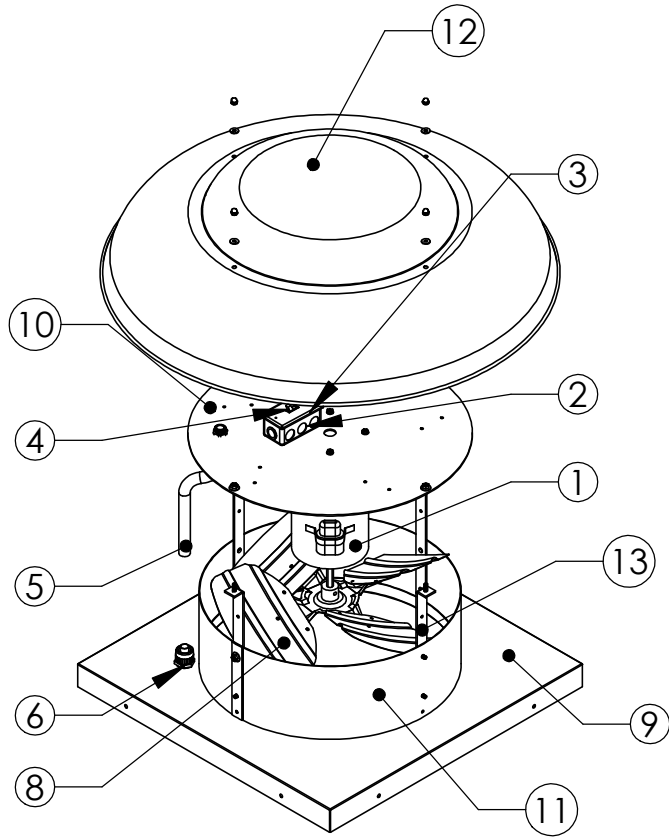
Direct Drive - Down Blast Axial Fan - Motor Information.
